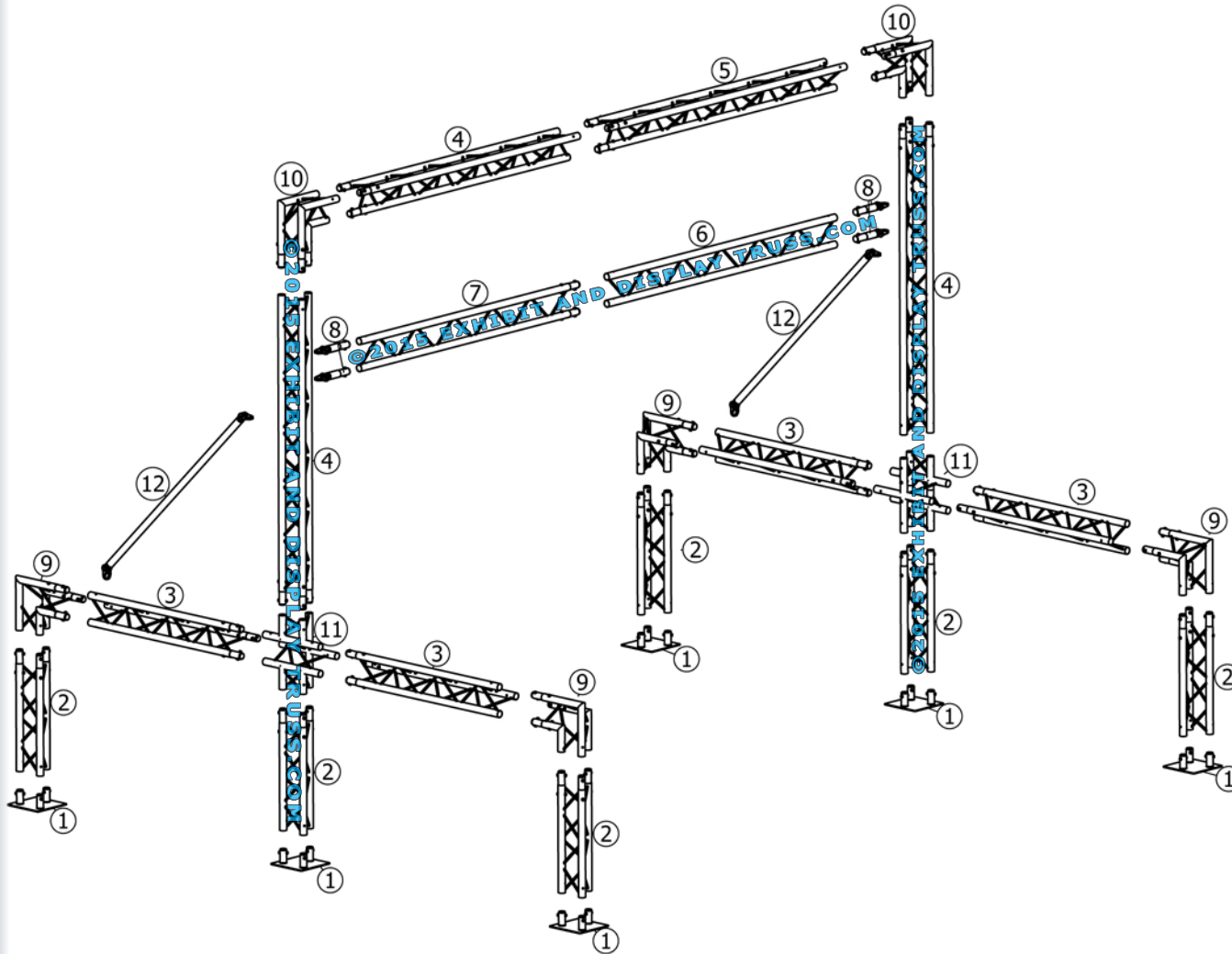
EXPLODED VIEW
