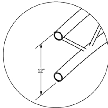
Curved Ladder (flat) Truss
