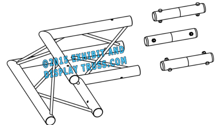
EXPLODED VIEW
