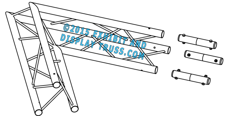
EXPLODED VIEW
