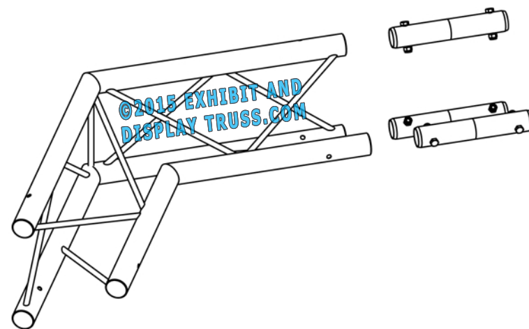
EXPLODED VIEW
