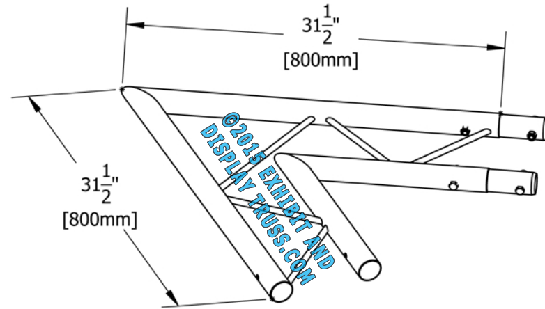
COLLAPSED VIEW
