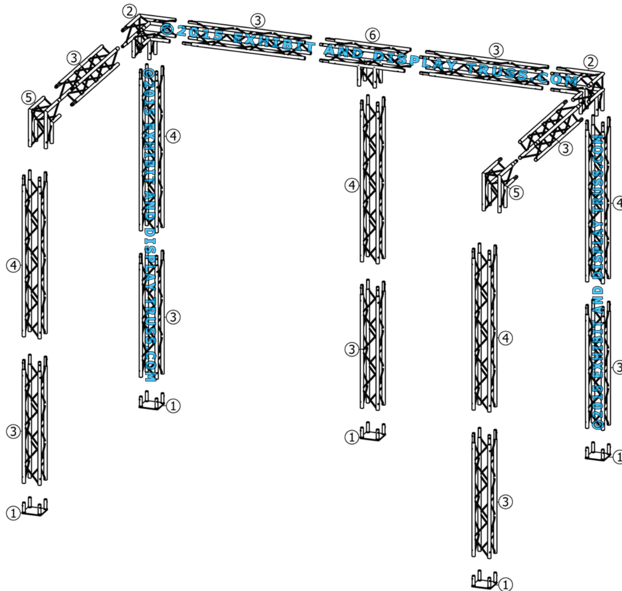
EXPLODED VIEW
