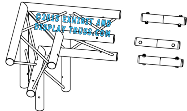
EXPLODED VIEW
