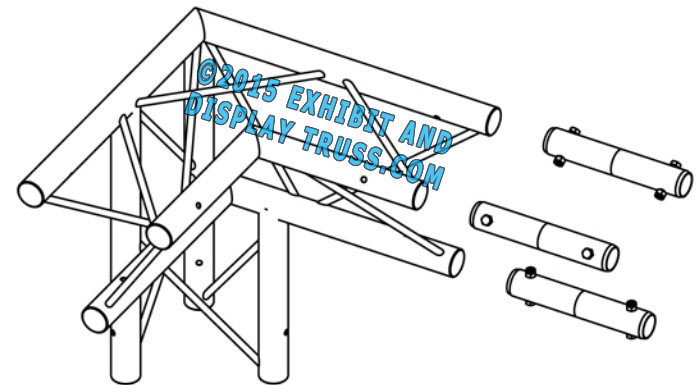
EXPLODED VIEW
