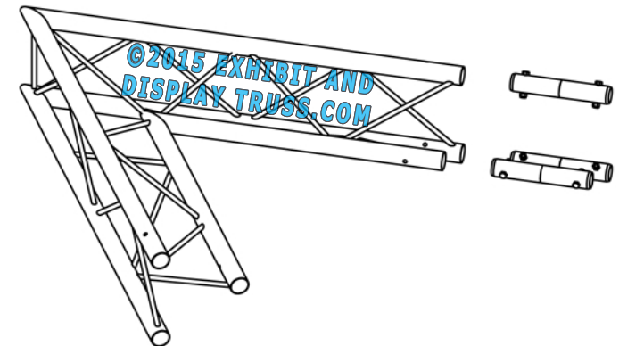
EXPLODED VIEW
