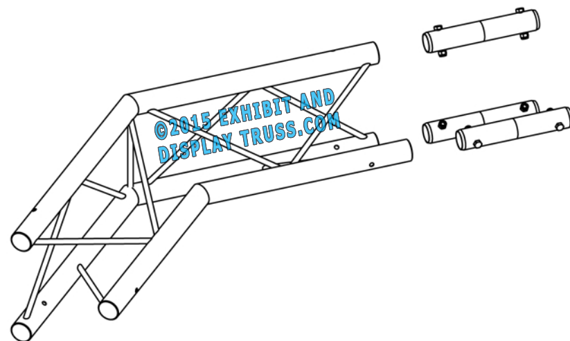
EXPLODED VIEW
