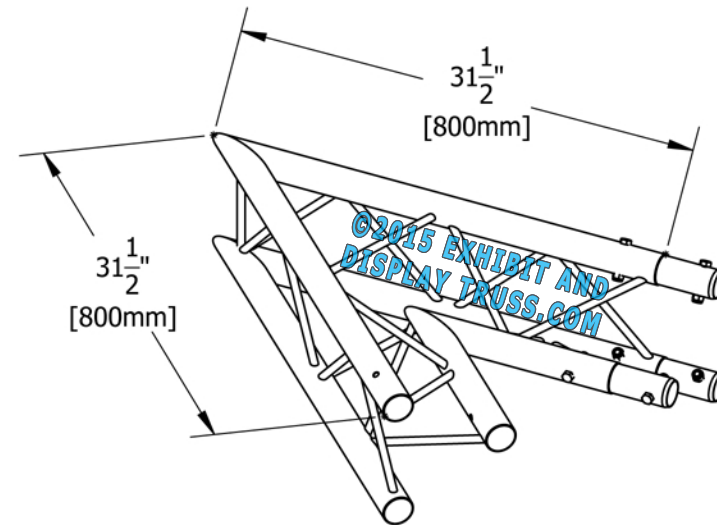
COLLAPSED VIEW
