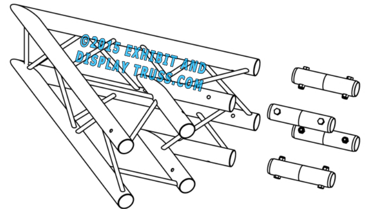
EXPLODED VIEW
