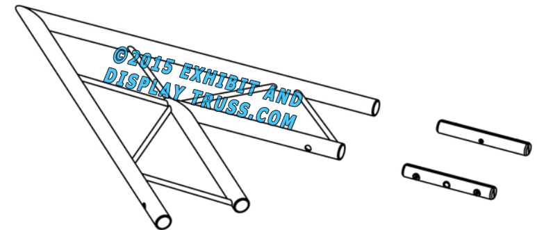
EXPLODED VIEW
